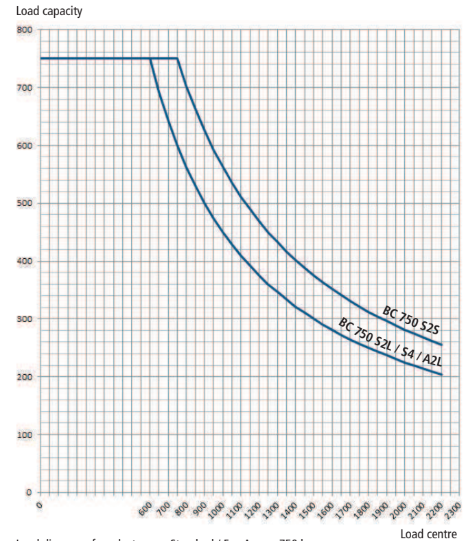
Load diagram of product group Standard / FreeAccess 750 kg
